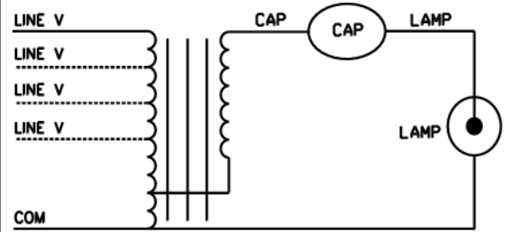
Wiring Diagram
