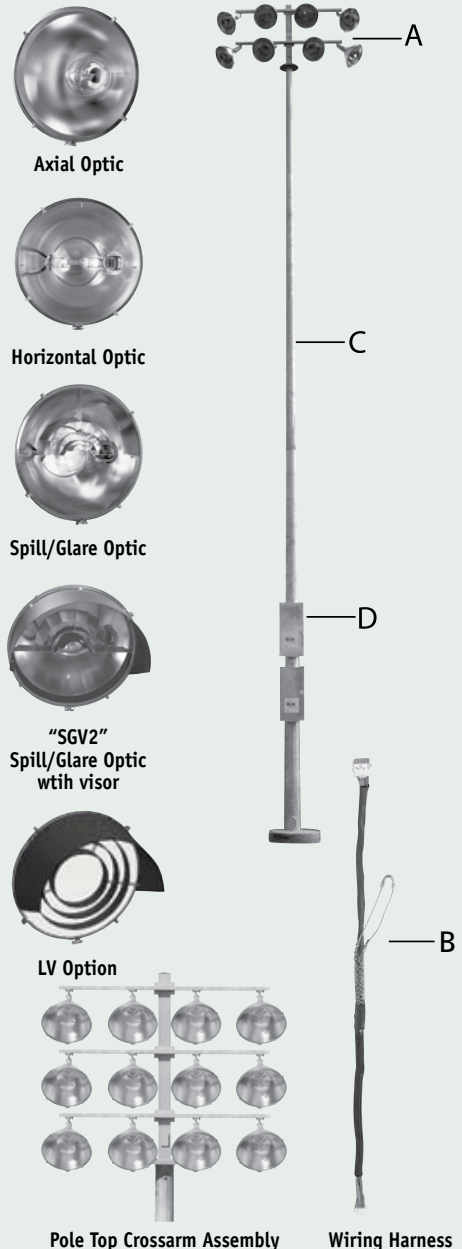
Pole Top Crossarm Assembly
